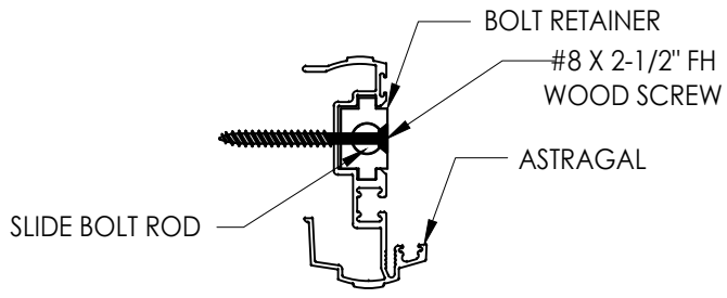
SECTION A-A Astragal Assembly
