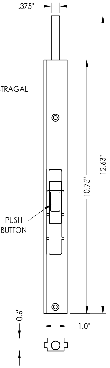
SLIDE BOLT ASSEMBLY (w/ Push Button) Aluminum
