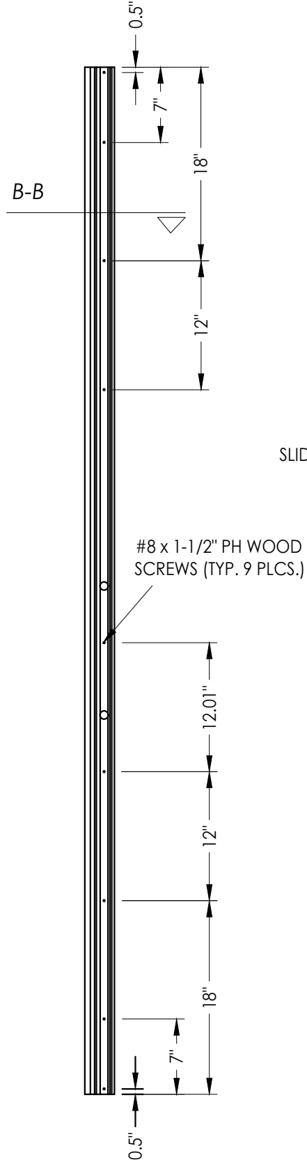
16 HURRICANE "T" ASTRAGAL by AFCO Aluminum
