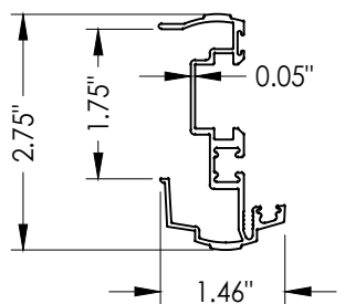
"T" ASTRAGAL PROFILE
