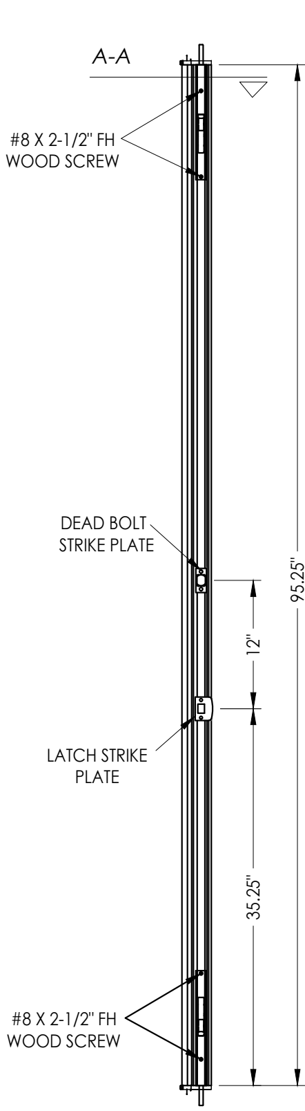
16 HURRICANE "T" ASTRAGAL by AFCO Aluminum
