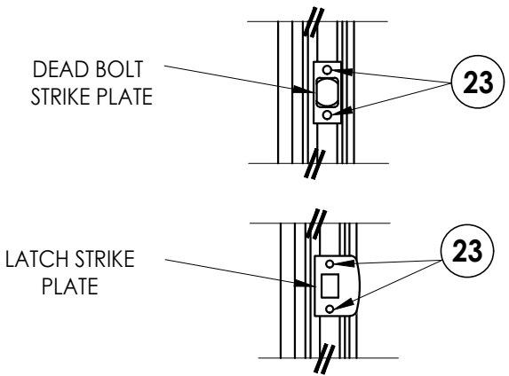
LATCH & DEAD BOLT DETAIL
